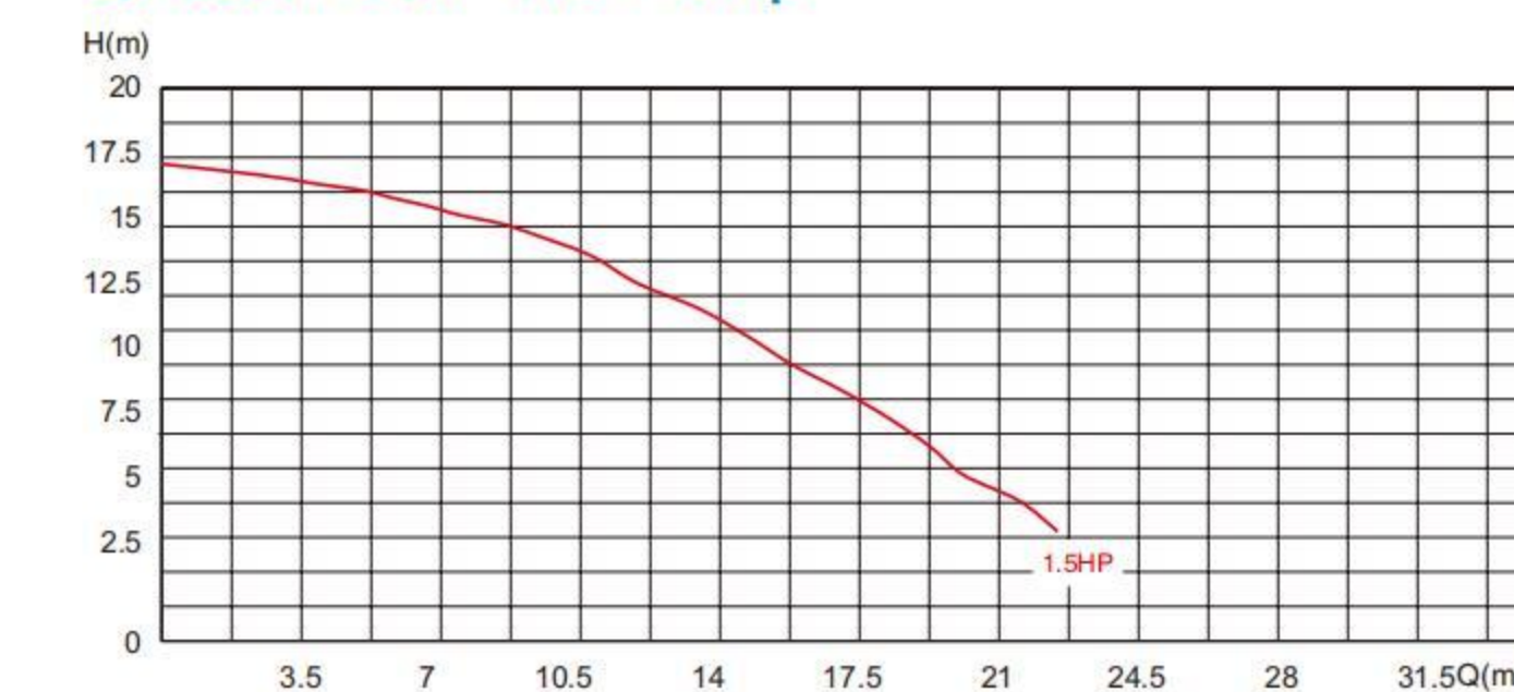
QH.Curve of The Pump
