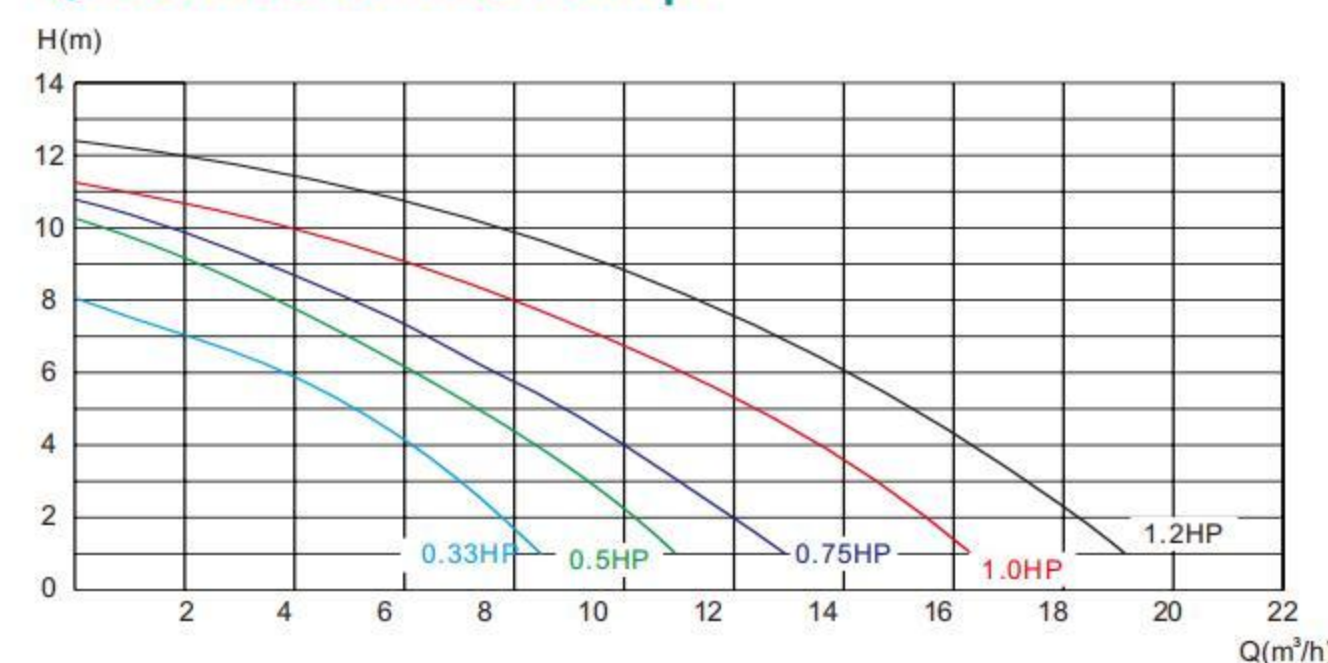
QH.Curve of The Pump
