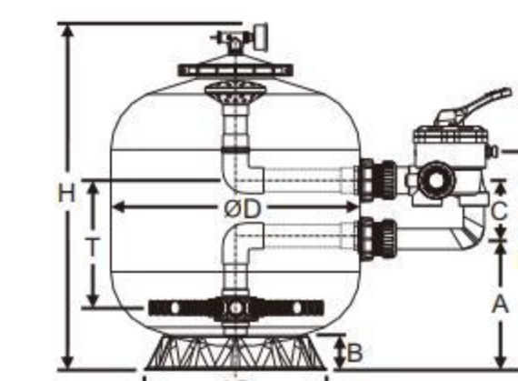
WL-BCG450~WL-BCG700
